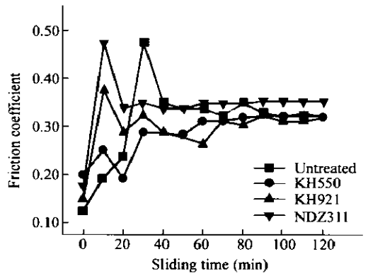
Fig. 1 Coupling agents versus the friction coefficient of the composites
