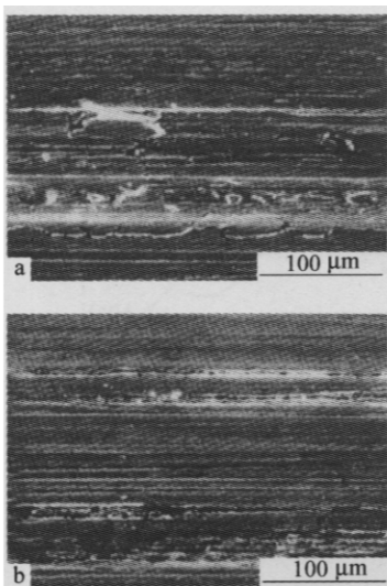
Fig. 4 SEM photographs of the transfer films of pure resin and TKw/BMI
